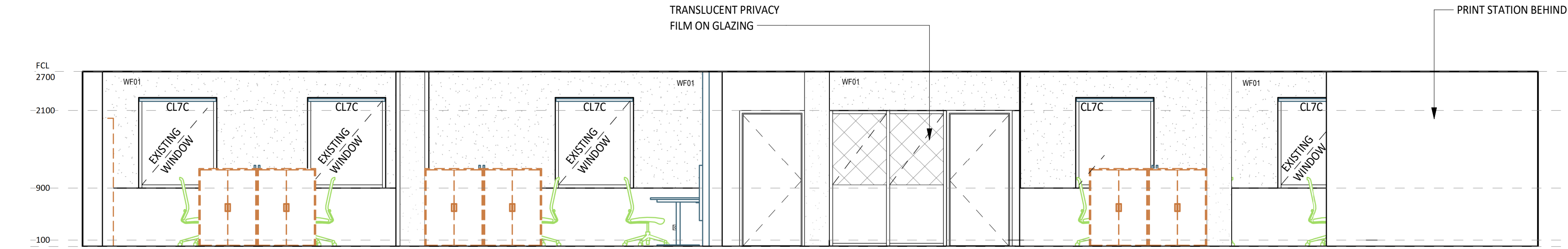
1 ELEVATION DETAIL 60-01 1:50
