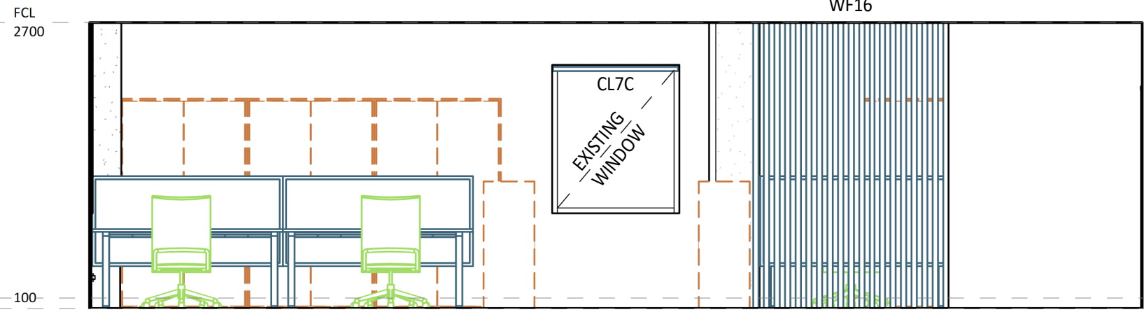
4 ELEVATION DETAIL 60-01 1:50
