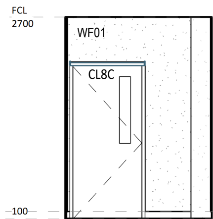
10 ELEVATION DETAIL 1:50
