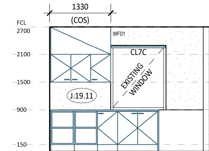
7 ELEVATION DETAIL 1:50
