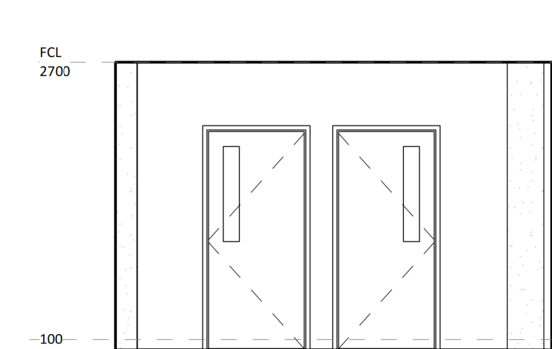
8 ELEVATION DETAIL 1:50
