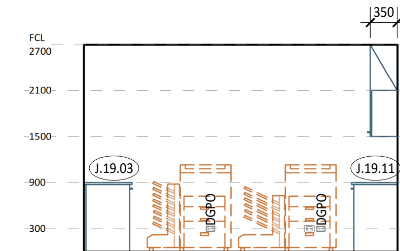
6 ELEVATION DETAIL 1:50
