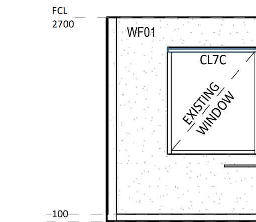
11 ELEVATION DETAIL 1:50
