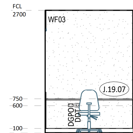
12 ELEVATION DETAIL 1:50
