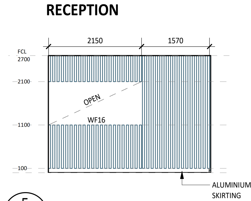
5 ELEVATION DETAIL 60-01 1:50
